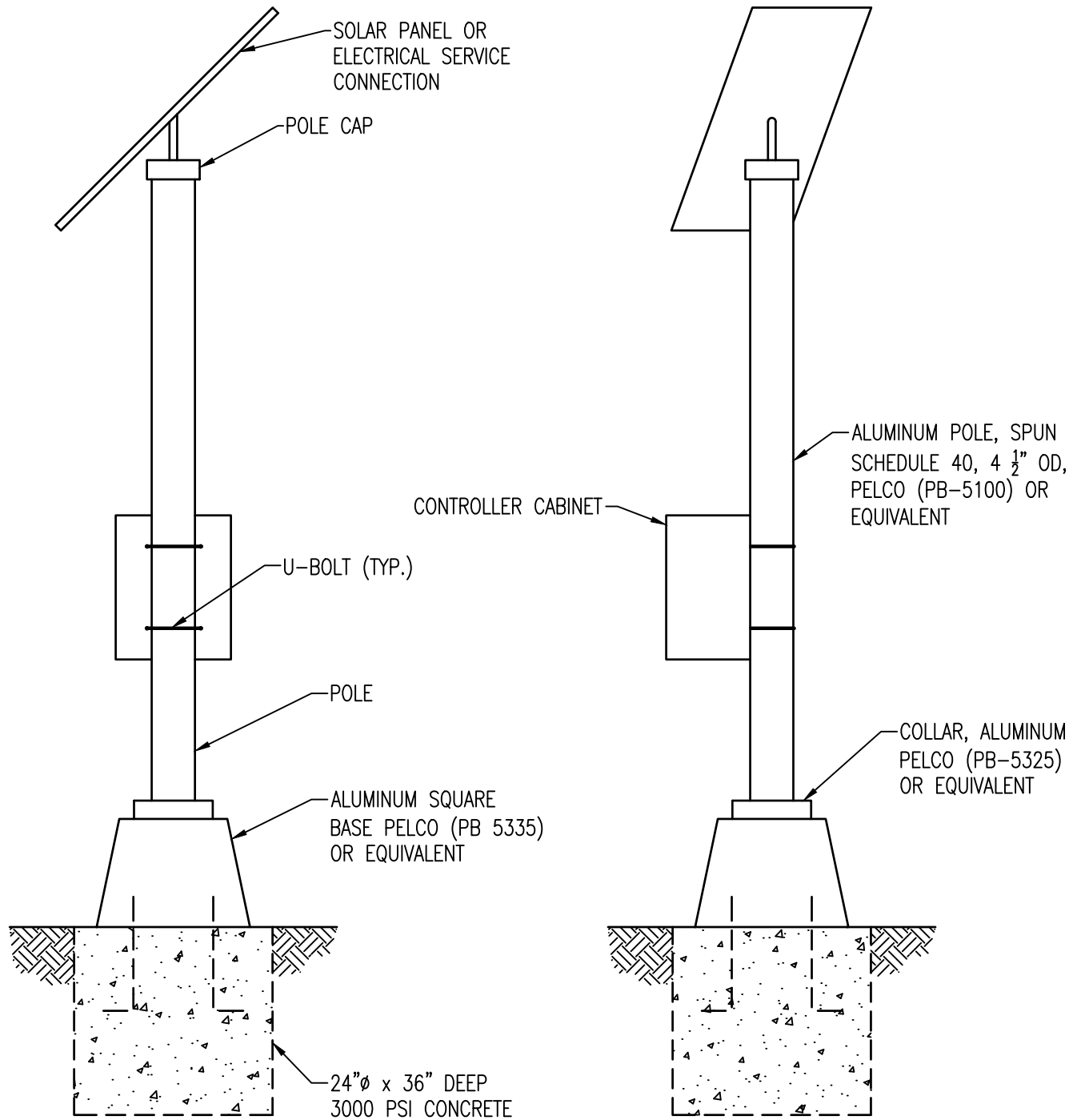
FRONT VIEW
