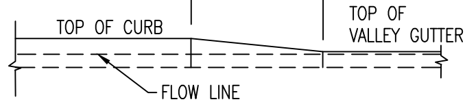
CURB TRANSITION – ELEVATION VIEW N.T.S.
