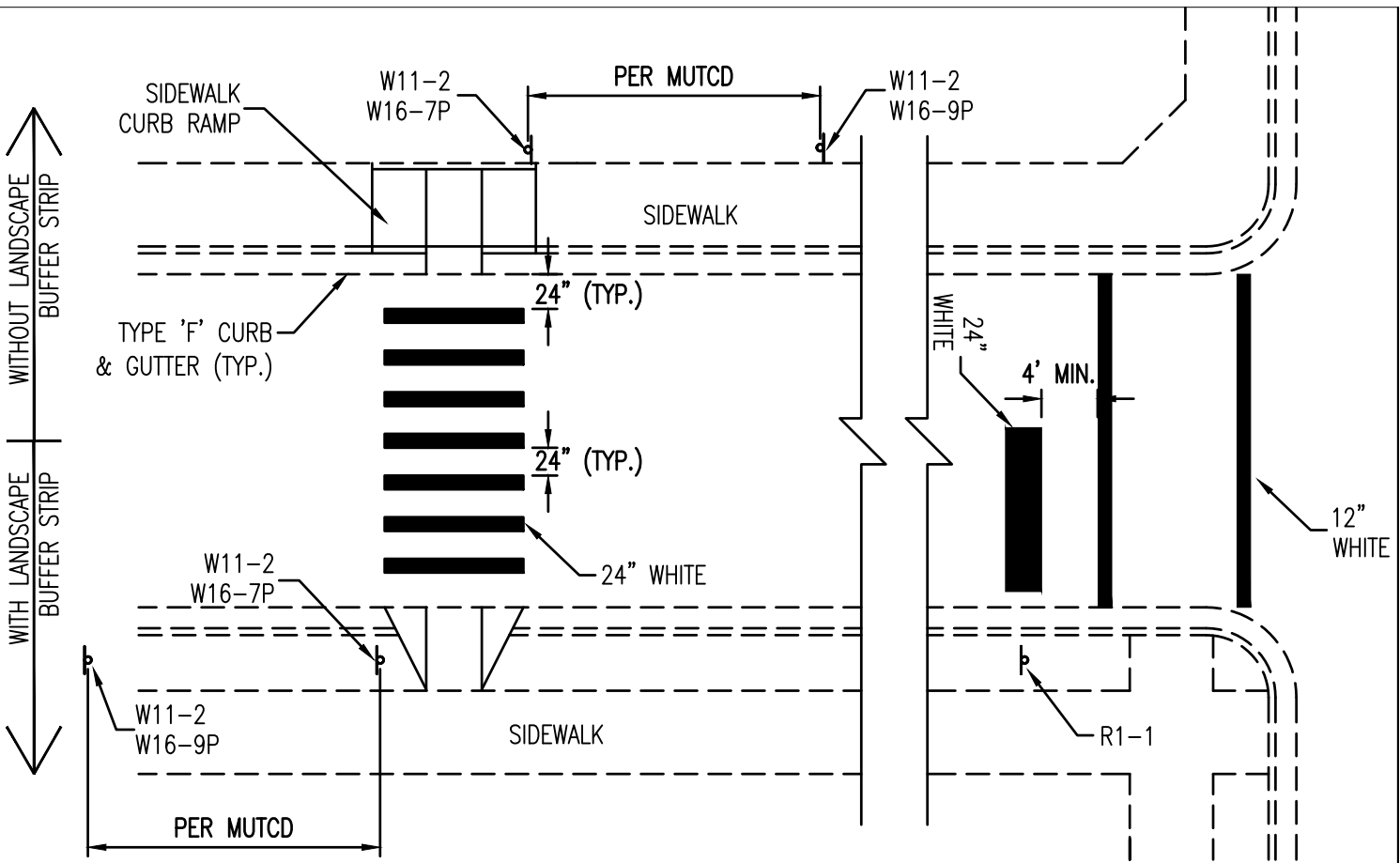
MID-BLOCK CROSSWALK
