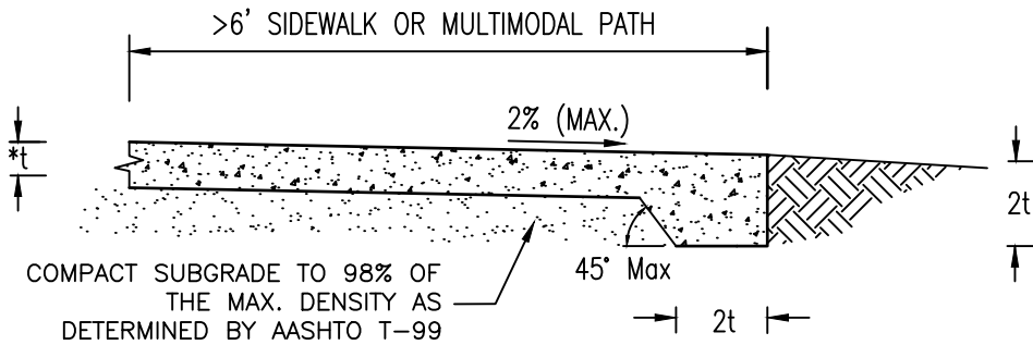
TYPE "D" CURB & SIDEWALK COMBINATION N.T.S.
