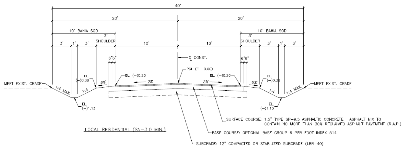
TYPICAL SECTION
