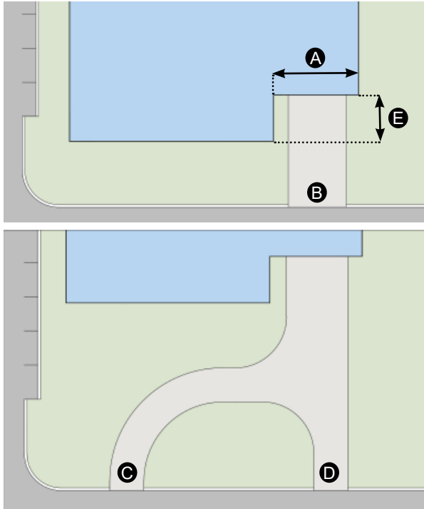
Figure 12-9.02 - Single Family Residential - Front Loaded - Side Entry
