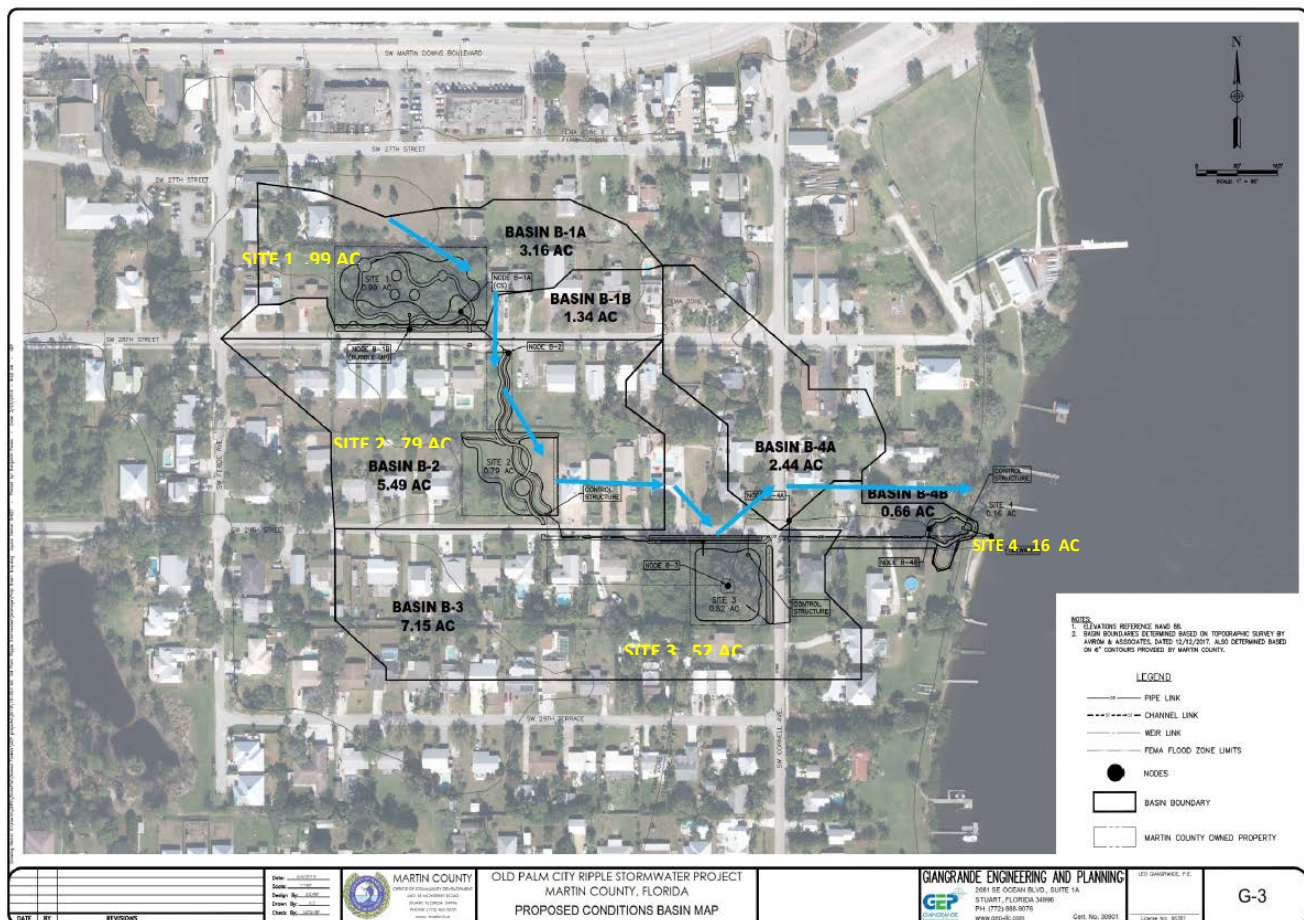
Figure 2: Stormwater Water Quality Retrofit Project Water Flow
